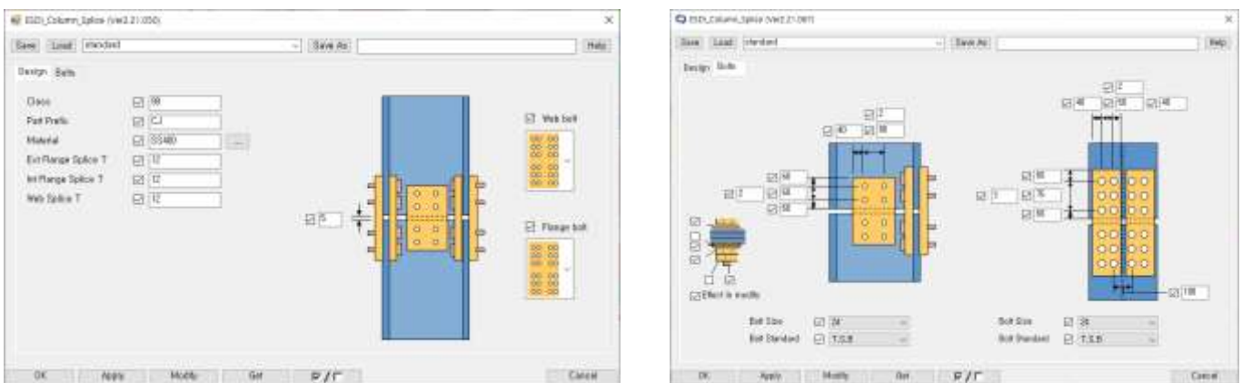
[ "Column Splice Connection" 화면 ]
