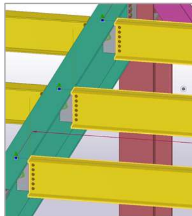
[Far Side Option 적용]
